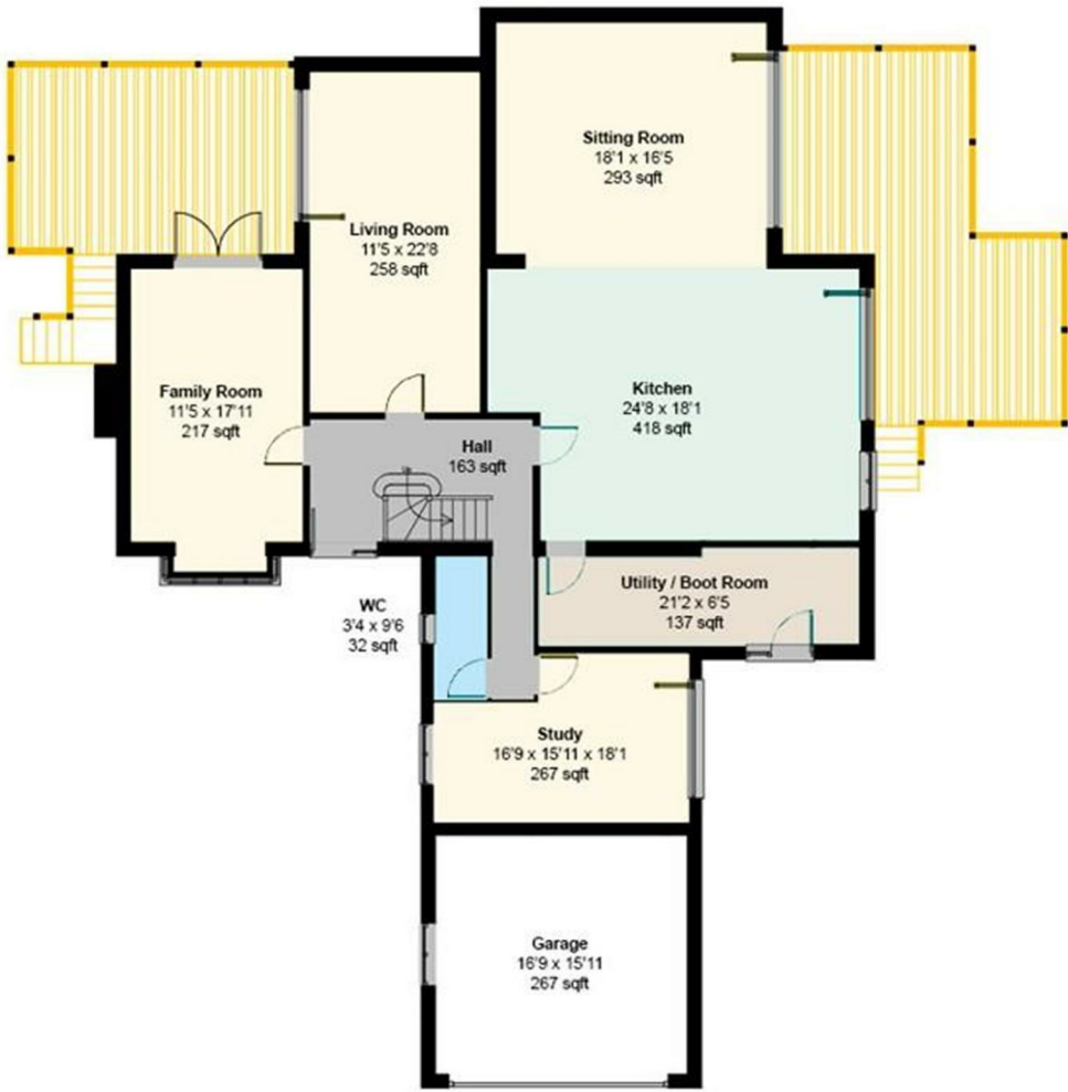
Ground Floor Exterior Area 1,928 sqft inc.garage
